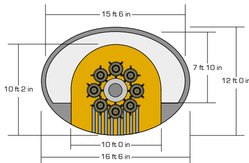
SM-73 WEAPON BAY CROSS SECTION
