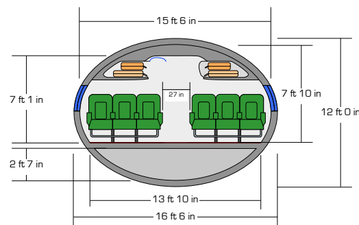
SM-74 CABIN CROSS SECTION
