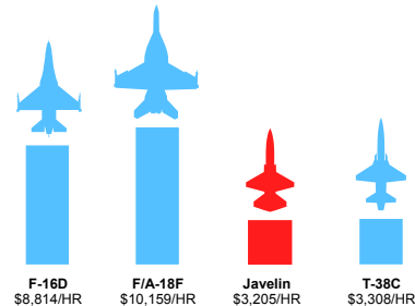
Javelin T-X Cost Per Flight Hour (CPFH) Comparison Non-Stavatti CPFH from FMS User Rates: DoD FY 2015 Reimbursable Rates Fixed Wing
